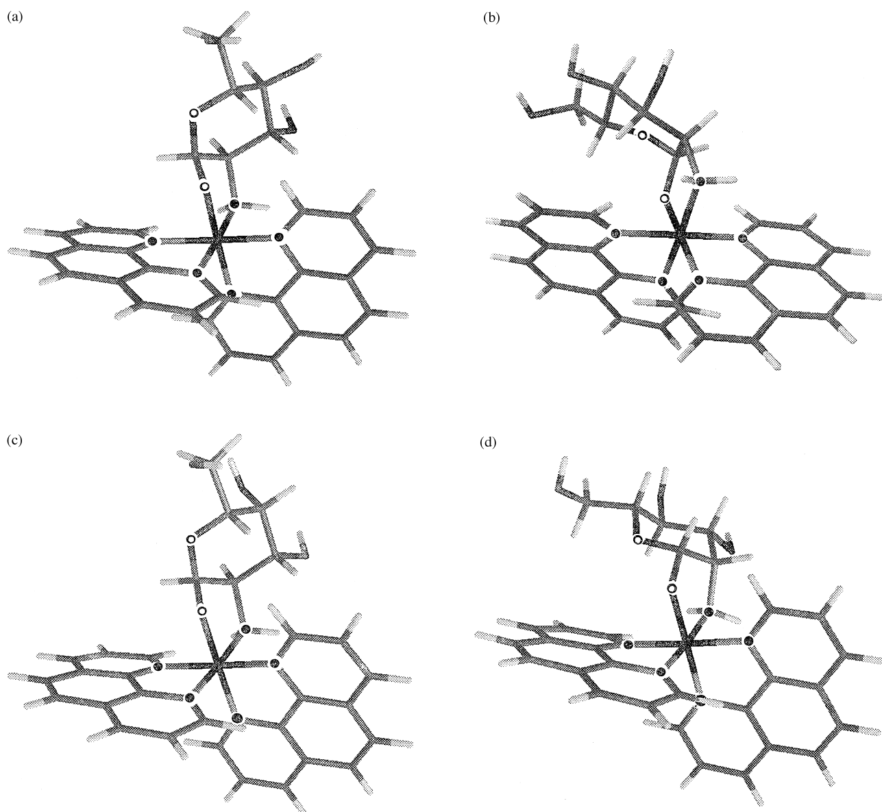
Fig. 1. Simulated (PM3-tm) structures of the dicationic Co(III) complexes, from the upper left: (a) \Delta -D-glucosamine Co(III) (phen)_2 ; (b) \Delta -D-glucosamine Co(III) (phen)_2 ; (c) \Delta -D-galactosamine Co(III) (phen)_2 ; (d) \Delta -D-mannosamine Co(III) (phen)_2 . In the \Delta -complexes oxygen-1 is in front of the plane of the paper, in the \Lambda -complex it is behind.
